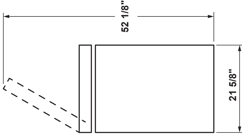
SIDE VIEW
